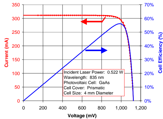
Figure 14. Measured Results for the GaAs Cell Without the Mini-Dome Lens
