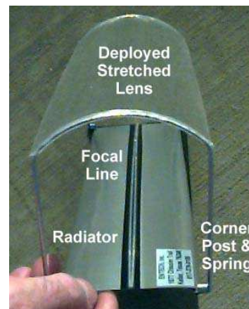
FIGURE 4. Stretched Lens Approach.
