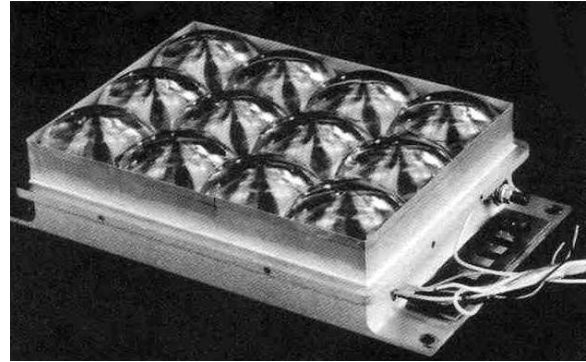
FIGURE 1. Mini-Dome Lens Array for PASP Plus (1994-1995).
