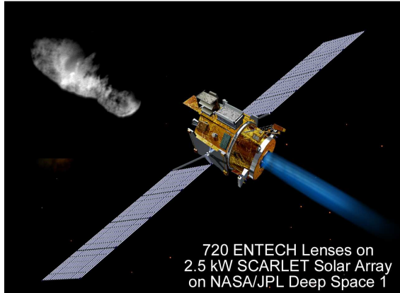
FIGURE 2. SCARLET Array on Deep Space 1 (1998-2001).
