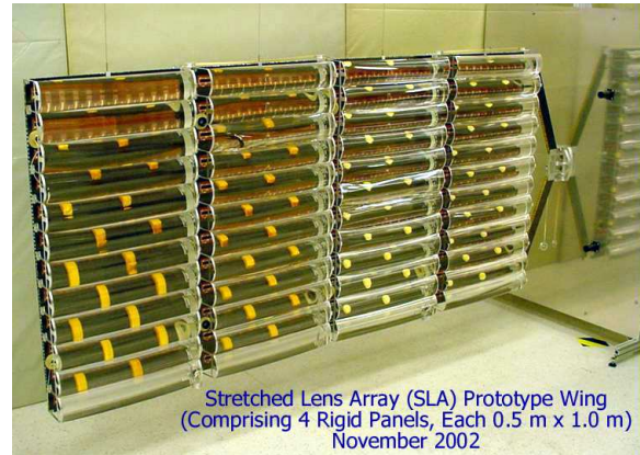
FIGURE 3. Rigid-Panel Stretched Lens Array (SLA) Wing.
