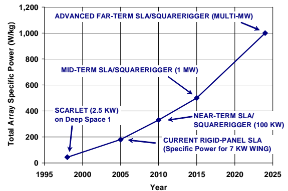
Figure 8. Long-Term Technology Roadmap for the Stretched Lens Array (SLA)
