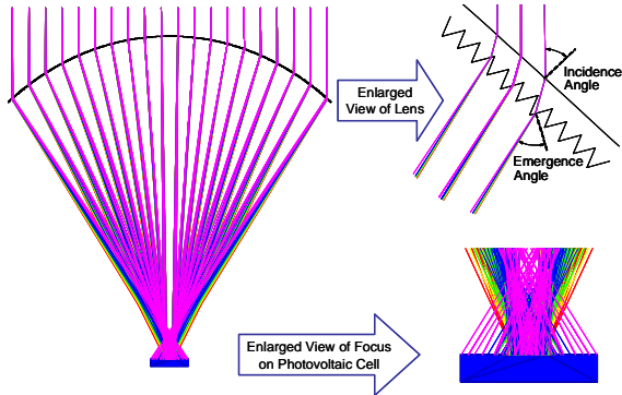
FIGURE 5. Symmetrical-Refraction Fresnel Lens.
