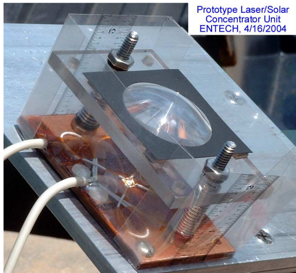
Figure 10. Improved Prototype Mini-Dome Lens GaAs Cell Photovoltaic Concentrator several other electrical, thermal, and mechanical improvements over the earlier module of Fig. 9.
