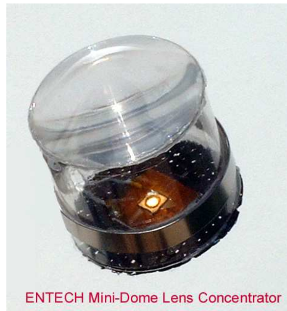
Figure 9. Mini-Dome Lens GaAs Cell Module
